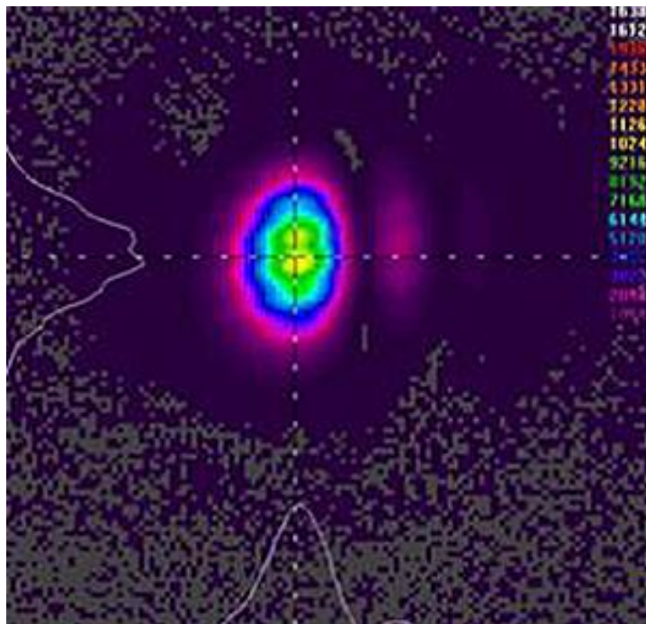
2-D Beam Profile at 1524.0 mm (60.0 in)
