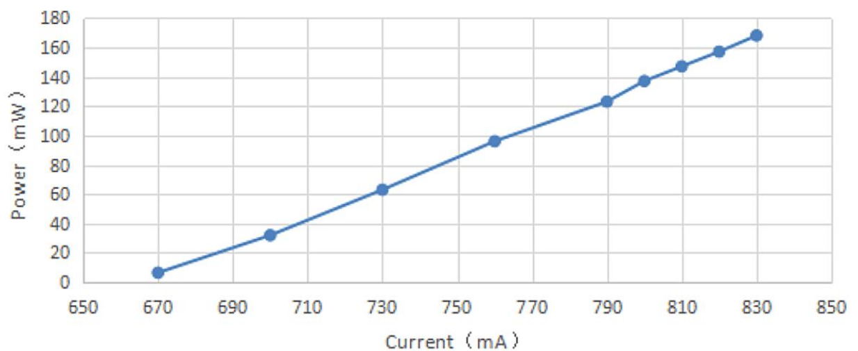
P-I tuning Curve
