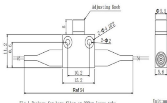
Fig.1 Package for bare fiber or 900um loose tube. The Color of Tube is Red.
