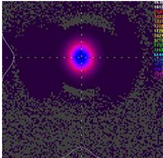
2-D Beam Profile at 1778.0 mm (70.0 in)
