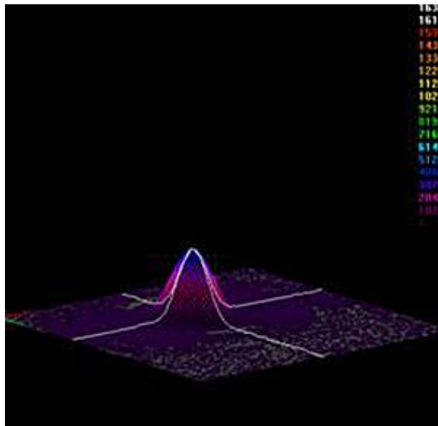
3-D Beam Profile at 1778.0 mm (70.0 in)
