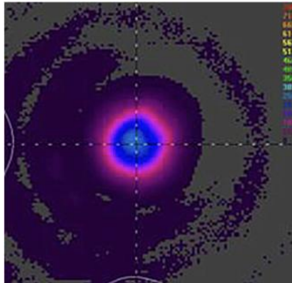
2-D Beam Profile at 1016.0 mm (40.0 in)
