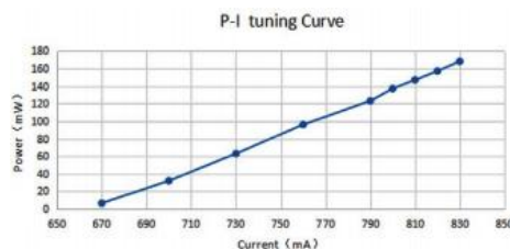
Power Stability of 4.0um FP-QCL Laser
