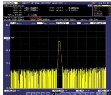
Laser Spectrum (Continuous)
